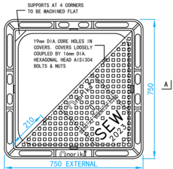
HALF COVER REMOVED TOP VIEW
